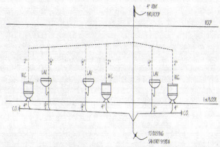
RISER DIAGRAM
